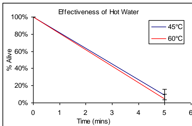
Figure A2.6: Effectiveness of 45°C and 60°C water in decontaminating Didymo on plastic
