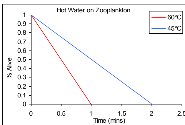
Figure A2.15: Effectiveness of hot water in decontaminating small aquatic invertebrates
