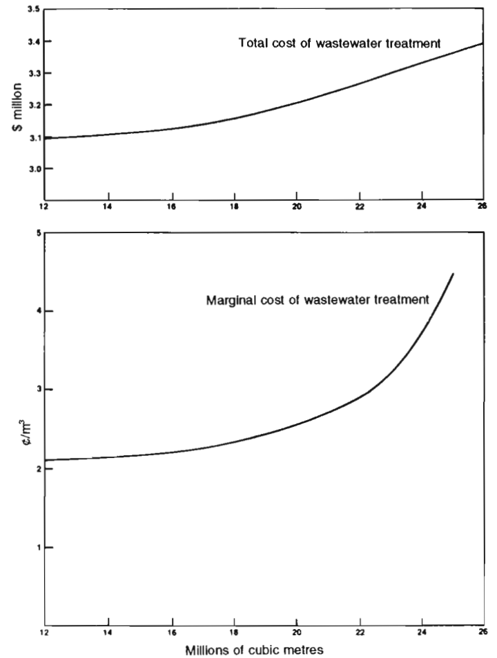
Figure 44. Marginal cost of wastewater treatment, derived from total cost curve, Case 2.
