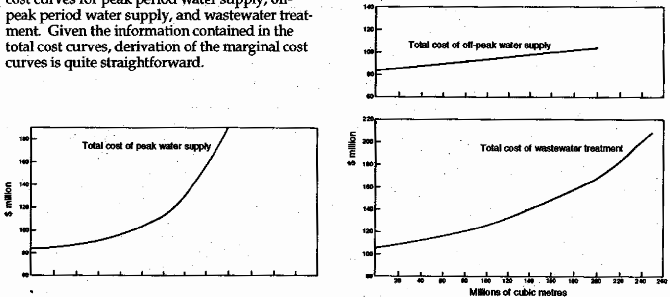
Figure 32. Total cost curves, Case 1.
