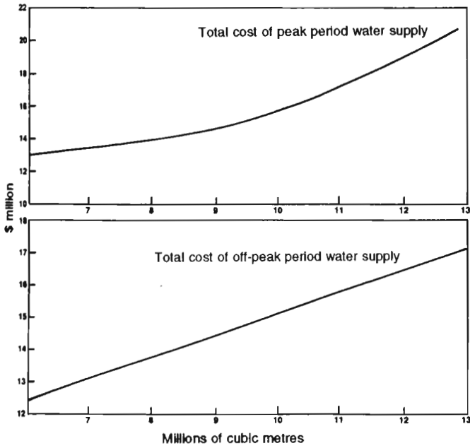
Figure 42. Total cost curves, Case 2.
