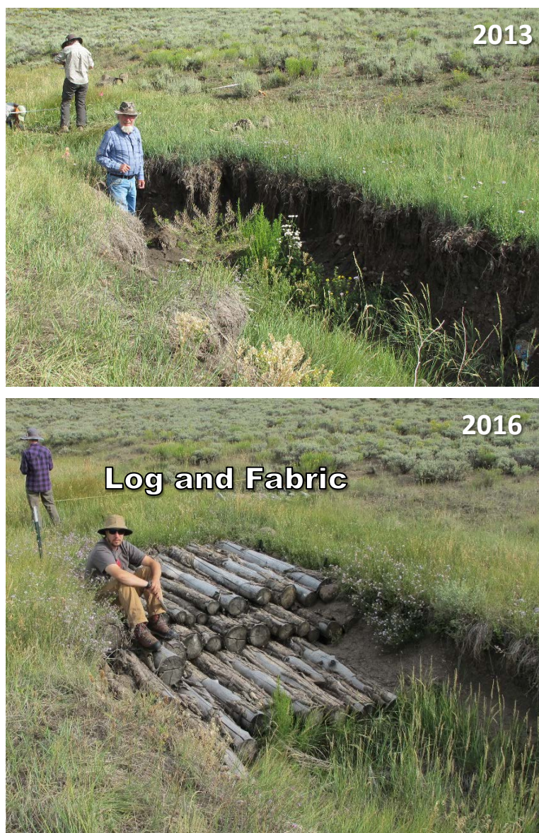
Figure 13. Log and fabric structure for treating headcuts before (top) and after (bottom) installation. Photos by: Renee Rondeau
