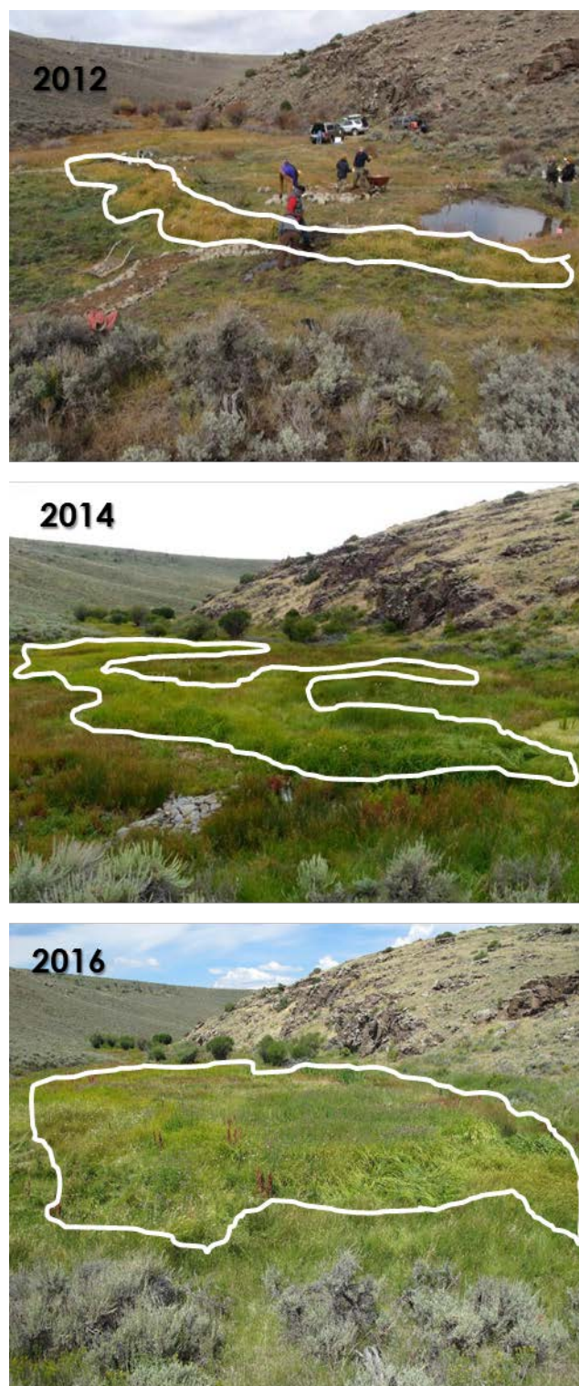
Figure 6. Extent of wetland vegetation before Zeedyk structures (2012) and 2-4 years post-treatment (2014 and 2016). White polygons represents the area supporting predominantly wetland vegetation. Photos by: Claudia Strijek (2012) and Renee Rondeau (2014, 2016)
